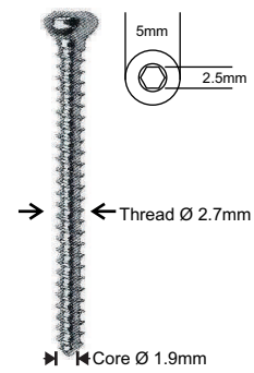
CORTEX SCREW Ø 2.7MM
