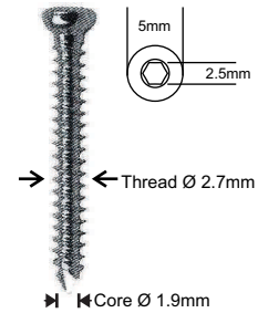
CORTEX SCREW Ø 2.7MM SELF TAPPING
