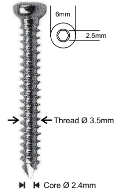
CORTEX SCREW Ø 3.5MM, SELF TAPPING
