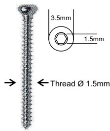
CORTEX SCREW Ø 1.5MM
