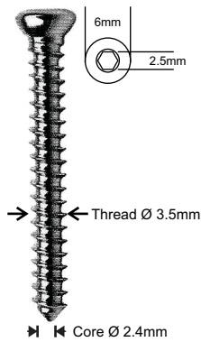
CORTEX SCREW Ø 3.5MM
