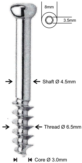
CANCELLOUS BONE SCREW Ø 6.5MM, 16MM THREAD
