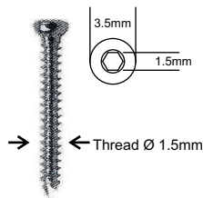
CORTEX SCREW Ø 1.5MM SELF TAPPING
