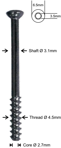
CORTEX CANCELLOUS SCREW Ø 4.5MM SHORT THREAD
