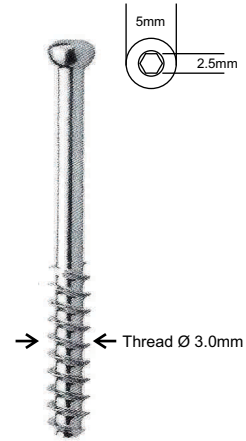
CANNULATED SCREW Ø 3.0MM SHORT THREAD
