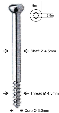
SHAFT SCREW Ø 4.5MM
