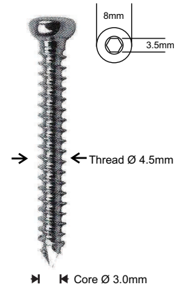
CORTEX SCREW Ø 4.5MM - SELF TAPPING
