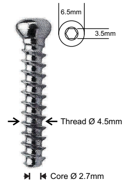
CORTEX CANCELLOUS SCREW Ø 4.5MM FULL THREAD
