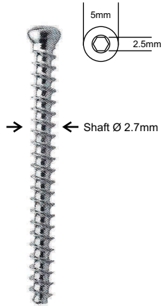
CORTEX CANNULATED SCREW Ø 2.7MM FULL THREAD
